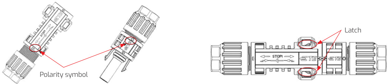
Fig. 7: Indication of polarity of the PV4-5 connectors Fig. 8: Mating the PV4-5 connectors
